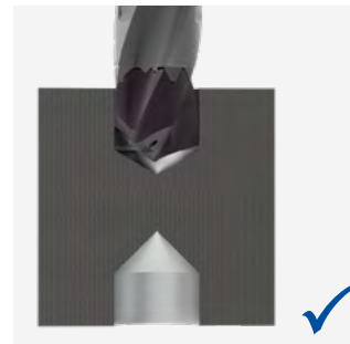
Breakthrough to bore in opposite direction; v_f = -50\%
